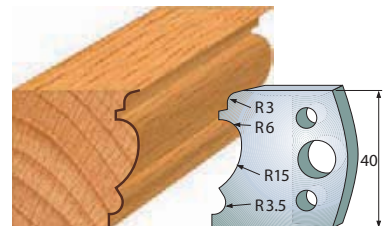
Pair of knives 690.104 Pair of limiters 691.104
