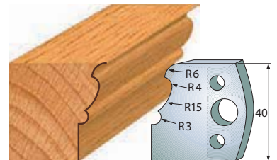
Pair of knives 690.101 Pair of limiters 691.101
