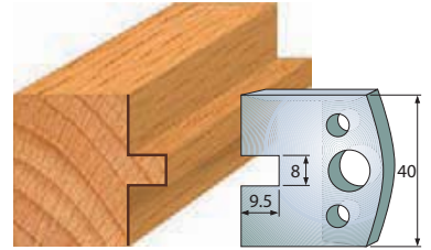
Pair of knives 690.095 Pair of limiters 691.095
