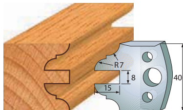
Pair of knives 690.099 Pair of limiters 691.099
